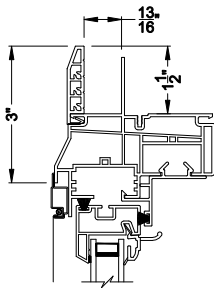
Z-FLANGE (1-1/2") Head Section Detail
