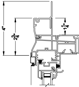
BRICKMOULD Head Section Detail
