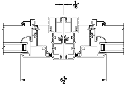
DIRECT MULL Jamb Section Detail
