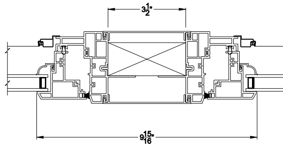
3-1/2" SPREAD MULL Jamb Section Detail
