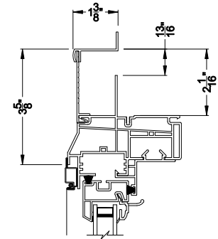
SIMULATED FLAT CASING Head Section Detail
