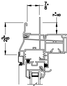
"J" CHANNEL Head Section Detail
