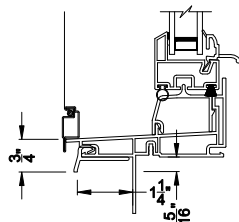
SILL NOSING Sill Section Detail
