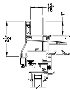
Z-FLANGE (1") Head Section Detail
