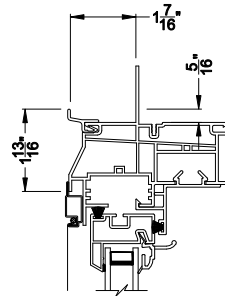
STUCCO ADAPTER Head Section Detail
