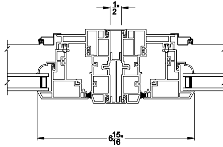
1/2" SPREAD MULL Jamb Section Detail
