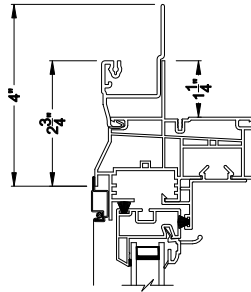
BRICKMOULD w/J-CHAN. Head Section Detail
