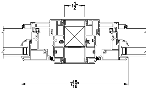
1-1/2" SPREAD MULL Jamb Section Detail
