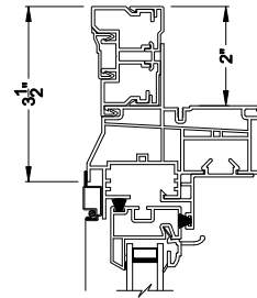
RENO. BRICKMOULD Head Section Detail
