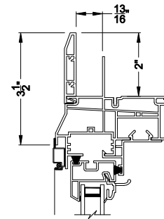
Z-FLANGE (2") Head Section Detail
