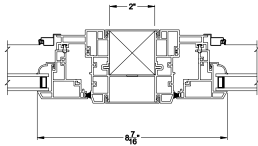
2" SPREAD MULL Jamb Section Detail
