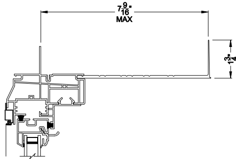
DRYWALL JAMB EXT. Head Section Detail
