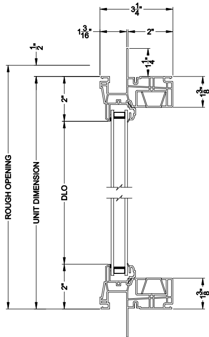
3500 PICTURE / TRANSM WINDOW (9311) Vertical Section - J-Channel
