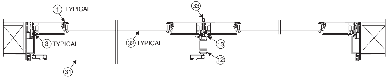
Centered Hinged 2 Panel Top View
