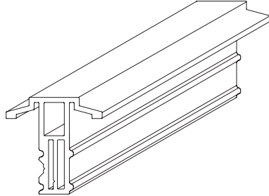
#11) Side Hinged Astragal Extrusion #5047
