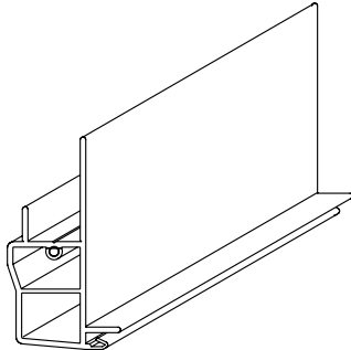
Brickmould for Outswing Doors Extrusion #1084
