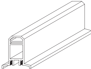
#26) Exterior Astragal (194.0) Extrusion #5031
