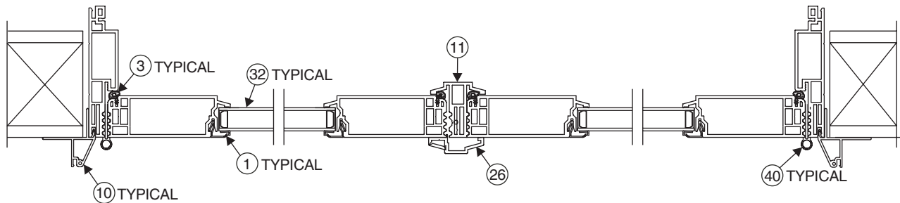
Side Hinged Outswing 2 Panel Top View
