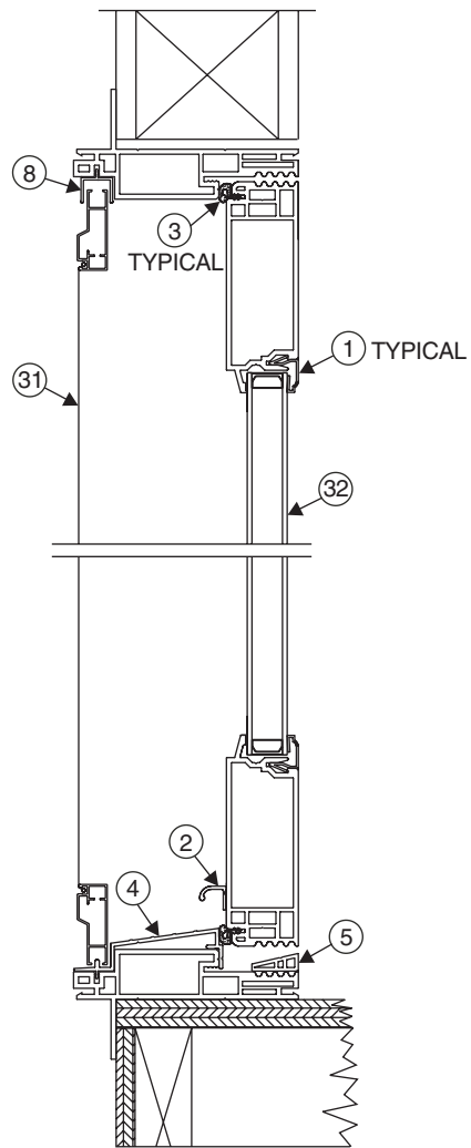
Center Hinged Side View
