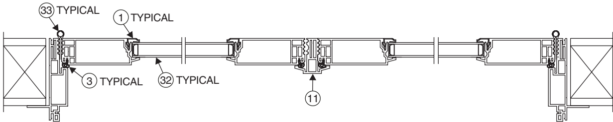
Side Hinged Inswing 2 Panel Top View
