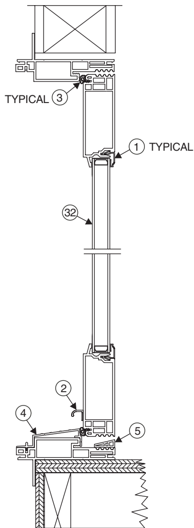
Side Hinged Inswing Side View
