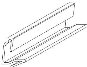
Brickmould for Outswing Doors Extrusion #1084
