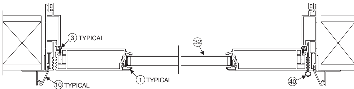
Side Hinged Outswing 1 Panel Top View
