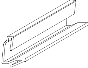
#1) Glazing Bead Extrusion #5041
