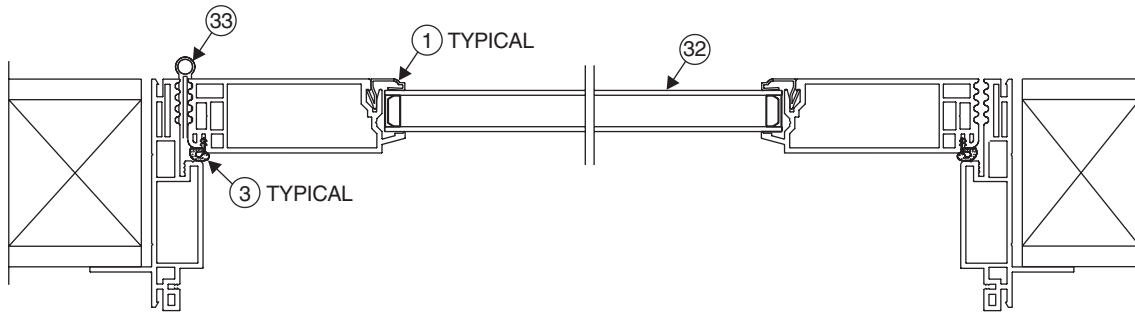
Side Hinged Inswing 1 Panel Top View
