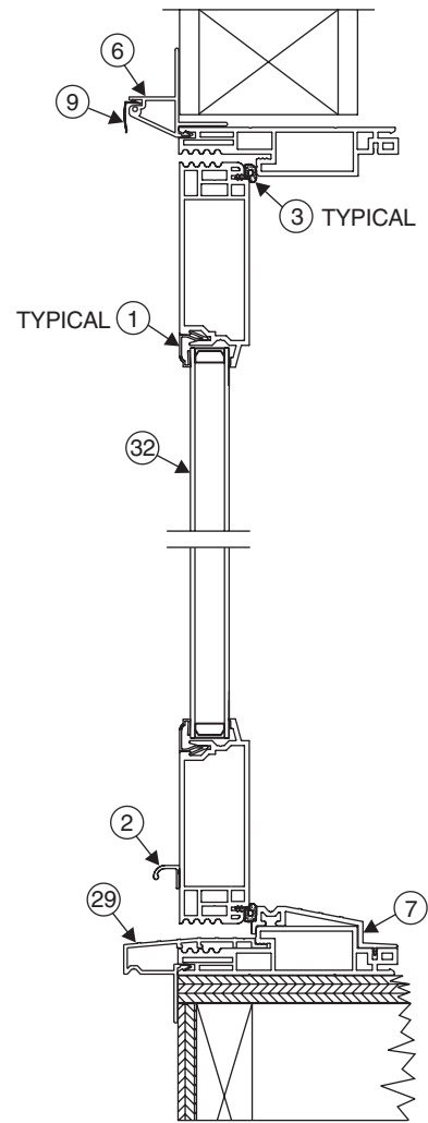
Side Hinged Outswing Side View
