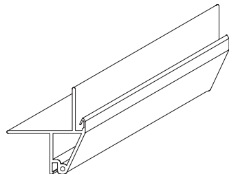
#6) Outswing TFT Extrusion #5030
